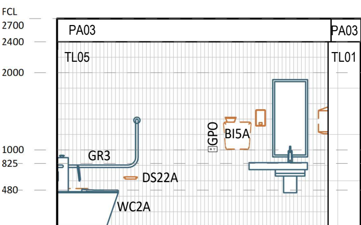
5 ELEVATION DETAIL 1 : 50
