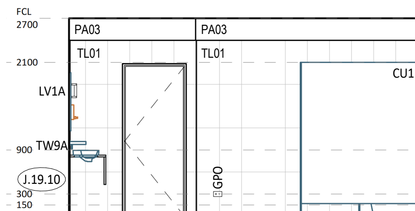
15 ELEVATION DETAIL 1 : 50
