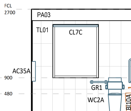
4 ELEVATION DETAIL 1 : 50
