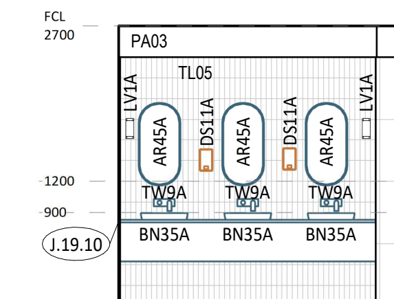
14 ELEVATION DETAIL 1 : 50
