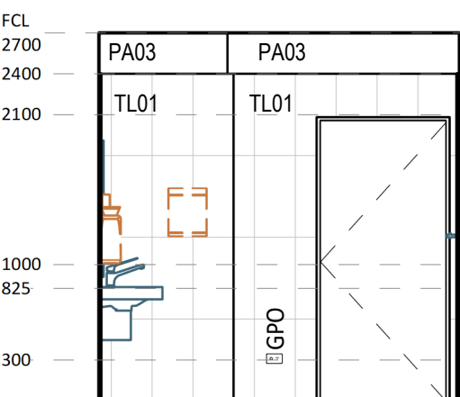
2 ELEVATION DETAIL 1 : 50
