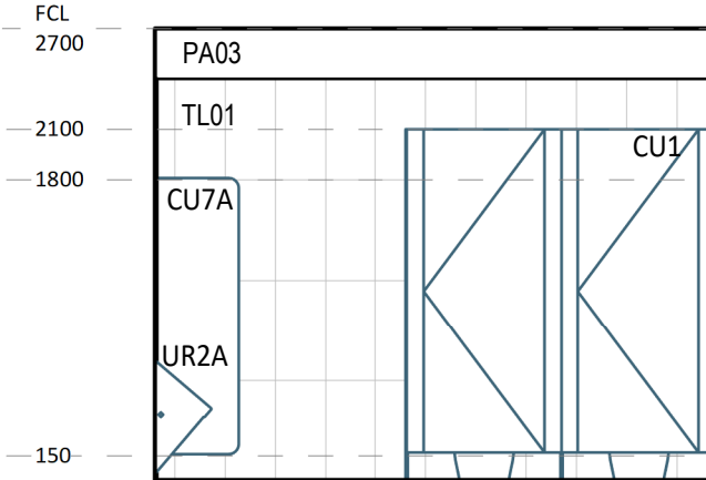
7 ELEVATION DETAIL 1 : 50
