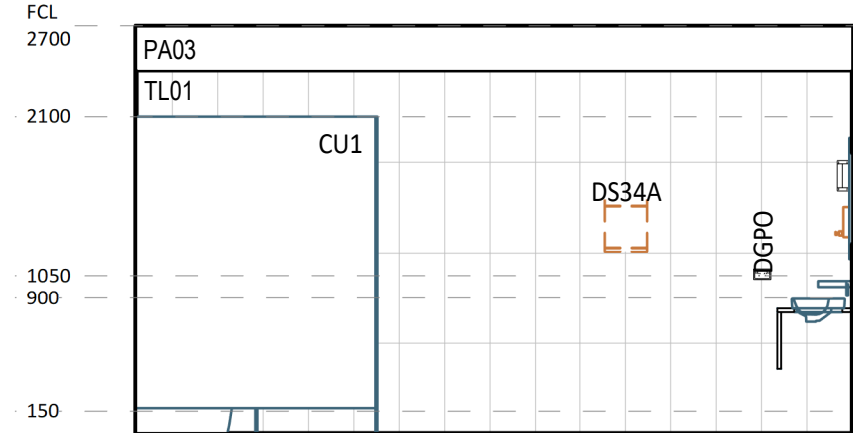
13 ELEVATION DETAIL 1 : 50
