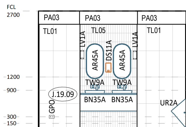
9 ELEVATION DETAIL 1 : 50
